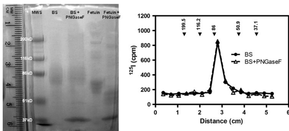
Fig. 3 Analysis of N-glycosylation status of the novel angiotensin binding site (representative results from three independent experiments). Left SDS-PAGE (7.5%) analysis and Coomassie blue staining of radio-photolabeled ( ^{125}\text{I} -SBpa-AngII), semipurified novel
