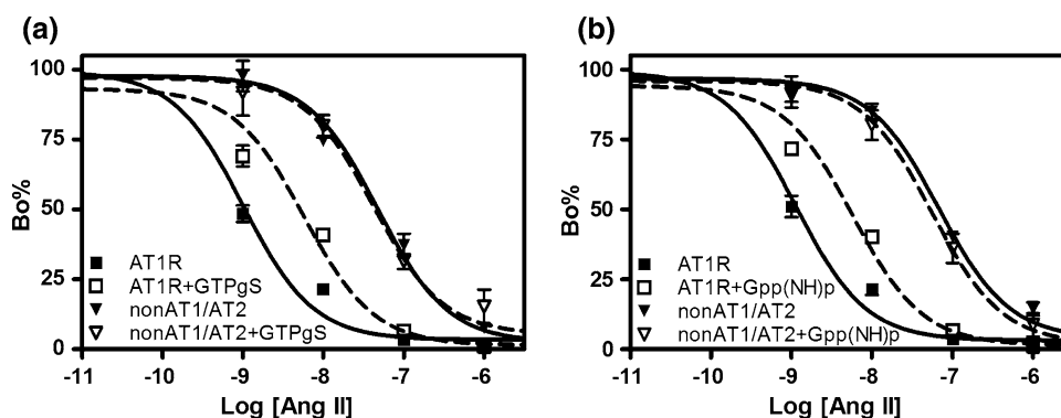
Fig. 5 Competition by Ang II for ^{125}\text{I} -SI Ang II ( \sim 0.25 nM) binding to the AT1 angiotensin receptor (AT1R; in liver membranes) or the novel angiotensin binding site (non-AT1/AT2; in cerebral cortical membranes) in the presence and absence of 50 \mu\text{M} GTP \gamma S (a) or 50 \mu\text{M} Gpp(NH)p (b); n = 3
