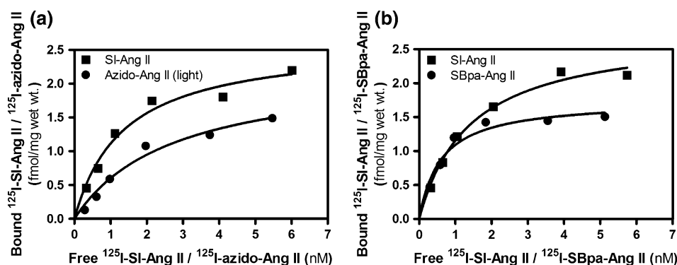
Fig. 1 High affinity binding of ^{125}\text{I} -azido-Ang II, ^{125}\text{I} -SBpa-Ang II, and ^{125}\text{I} -SI-Ang II to the novel angiotensin binding site in rat brain membranes. a Representative saturation analyses of ^{125}\text{I} -SI-Ang II ( B_{\max} = 2.6 \pm 0.2 fmol/mg wet wt, K_d = 1.35 \pm 0.3 nM) and ^{125}\text{I} -azido-Ang II ( B_{\max} = 2.24 \pm 0.3 fmol/mg wet wt, K_d = 2.7 \pm 0.78 nM) binding in rat cerebral cortical membranes in the presence of 10 \mu\text{M} PD123319, 10 \mu\text{M} losartan, and 0.3 mM PCMB (1 h
