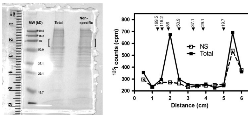
Fig. 2 Radiolabeling of the novel angiotensin binding site with photoaffinity probe ^{125}\text{I} -azido-Ang II in rat forebrain membranes (representative results from four independent experiments). Left SDS-PAGE (12%) analysis of radio-photolabeled rat forebrain membranes followed by Coomassie blue staining; bracketed areas represent a segment of the lanes (between molecular masses 86 and 50 kDa) corresponding to the highest specific binding (10 \mu\text{M} Ang II
