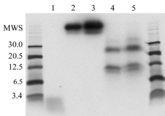
Fig. 4 Representative autoradiogram of Tris-tricine-SDS-PAGE (16.5%) analysis of CNBr and PNGaseF digests of radio-photolabeled ( ^{125}\text{I} -SBpa-AngII) and semipurified novel angiotensin binding site. Lane 1 contains free/unbound ^{125}\text{I} -SBpa-AngII, lane 2 contains untreated binding site, lane 3 contains PNGaseF-treated binding site, lane 4 contains CNBr-treated binding site, lane 5 contains CNBr and PNGaseF-treated binding site
